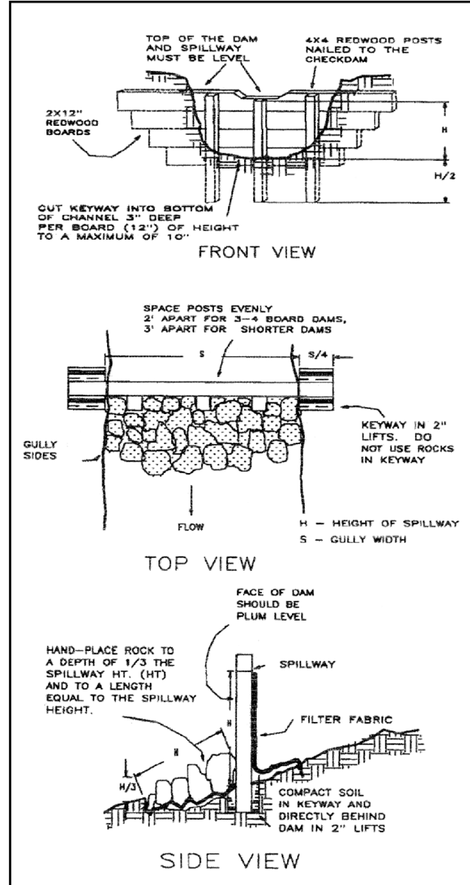
Figure 7. Redwood check-dam.
