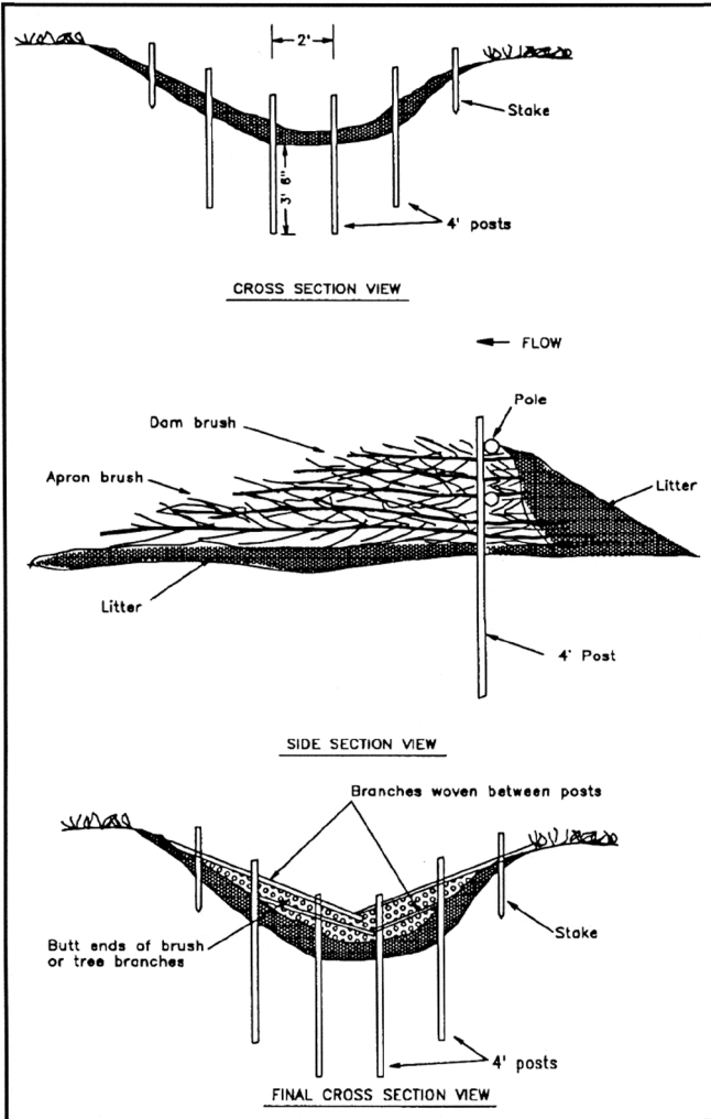
Figure 6. Post and brush dam.
