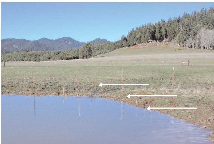
Figure 15. Pond with reshaped banks to reduce slope, planted with live staked willow and cottonwood (arrows).
